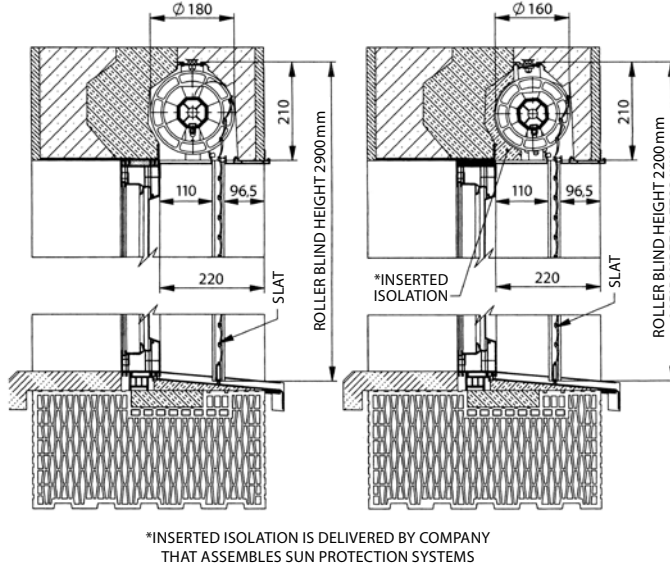
FITTING THE WINDOW FRAME FOR ROLLER BLINDS 220 mm FROM THE OUTSIDE LINING OF THE LINTEL
